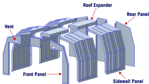
Components of a 10' Wide by 8' Long Enclosure
